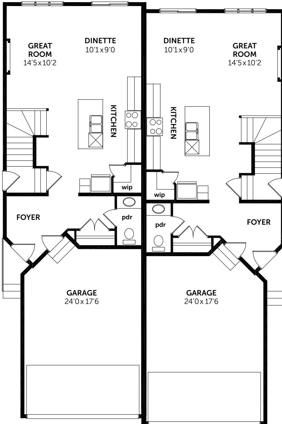
MAIN FLOOR 703 SF
