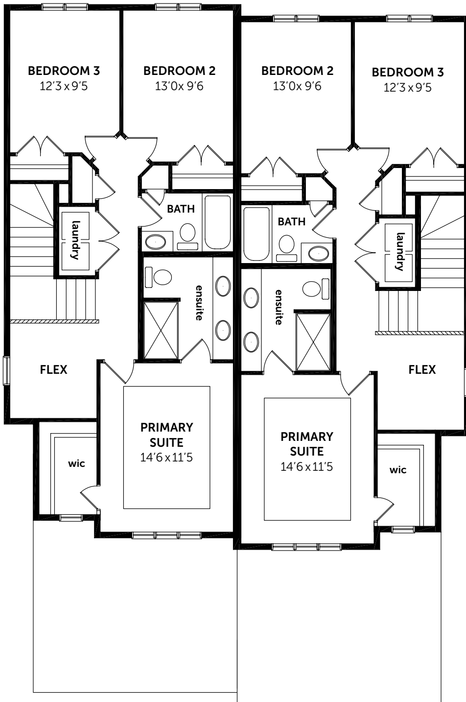
SECOND FLOOR 827 SF
