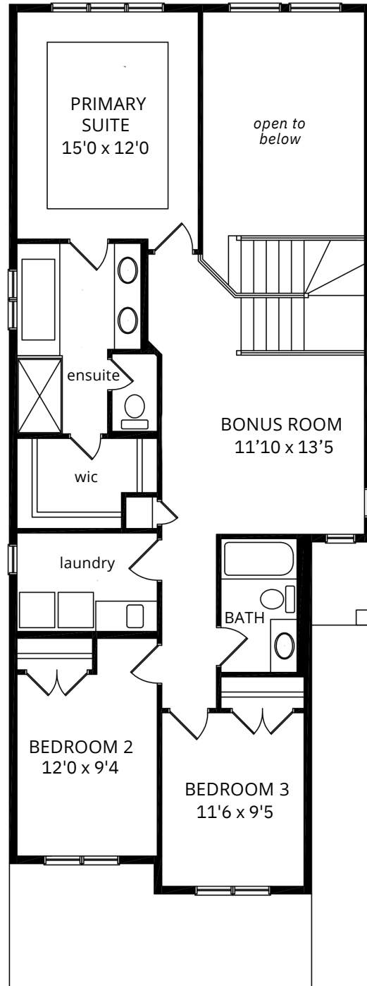
SECOND FLOOR 1,070 SF
